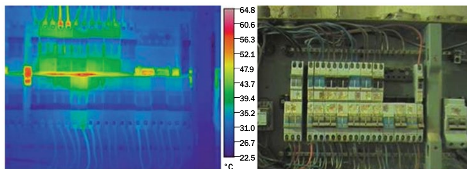
Figure 1.2. Thermographic picture of an electrical panel in a livestock barn.
