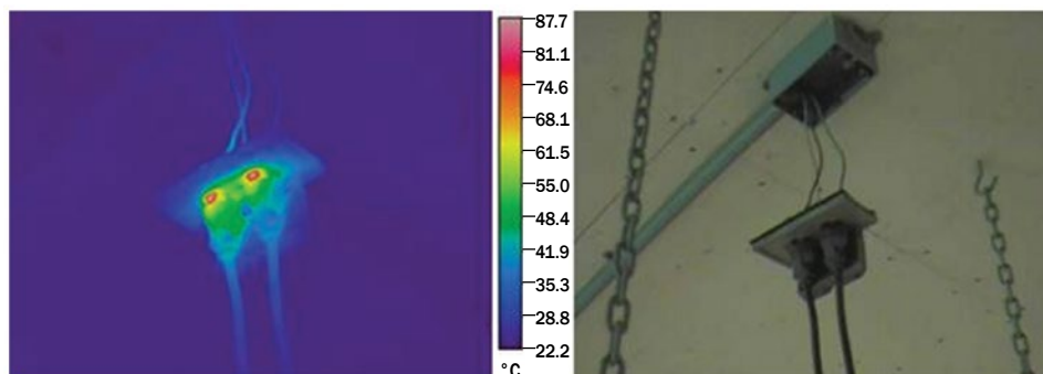
Figure 1.1. Thermographic picture of an electrical receptacle in a livestock barn.
